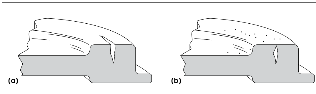
Figure 11. The effect of mechanical cleaning operations on discontinuities: (a) before mechanical cleaning; (b) after mechanical cleaning.
