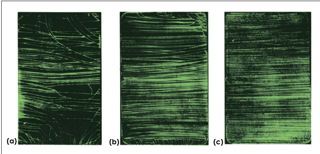
Figure 3. Fluorescent indications of stress cracks in chrome-plated nickel test panels: (a) coarse cracks; (b) medium cracks; and (c) fine cracks.
