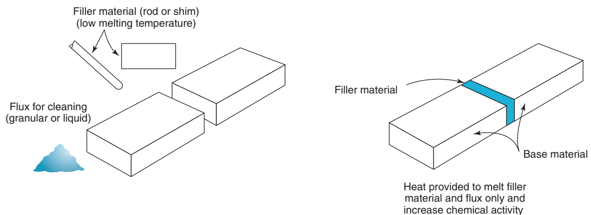
Figure 8.5: Flow bond.
