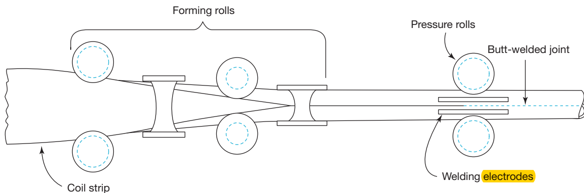
Figure 7.10: Resistance welding of tubing.
