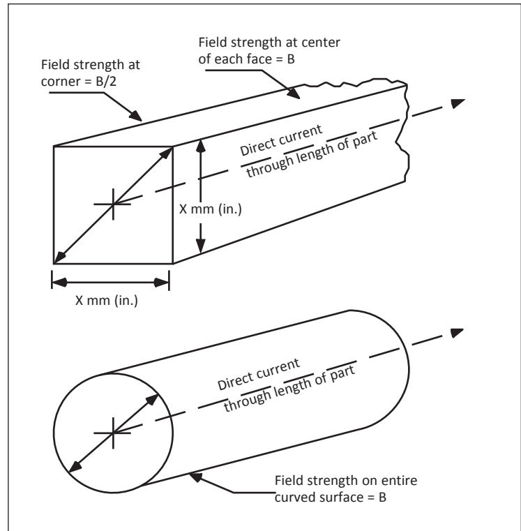
Figure 4.13: Field strength versus current. The diameter of the part is taken as the greatest distance between any two points on the outside circumference of the part.
